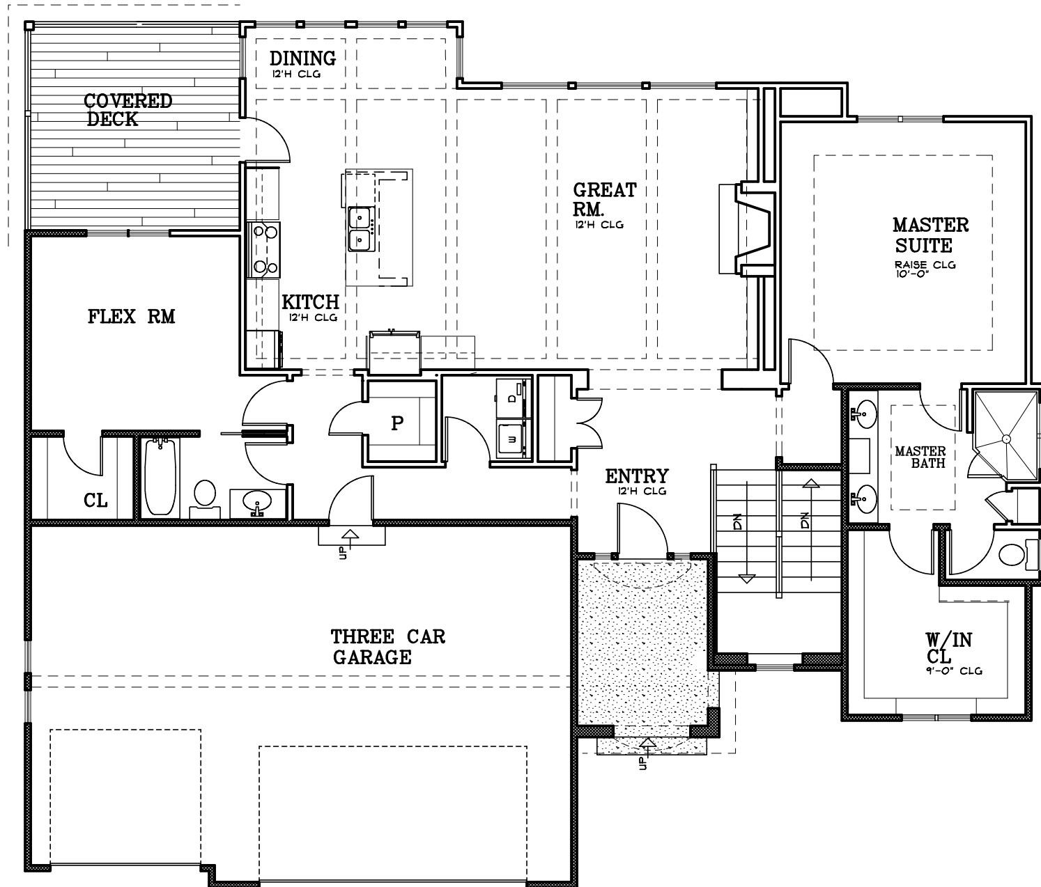
MAIN FLOOR PLAN AREA=1646 SQ FT
